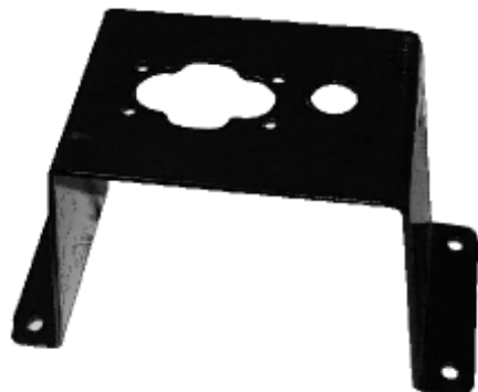
Air Shift Valve Low Mounting Tower #ASVT-05
