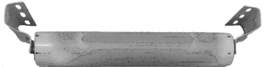
18" Return Idler c/w Brackets #18-10420R
