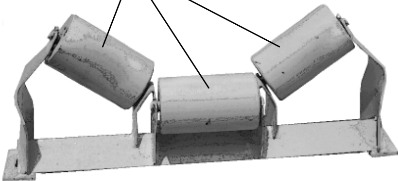
18" Troughing Idler Assembly #18-10402T
